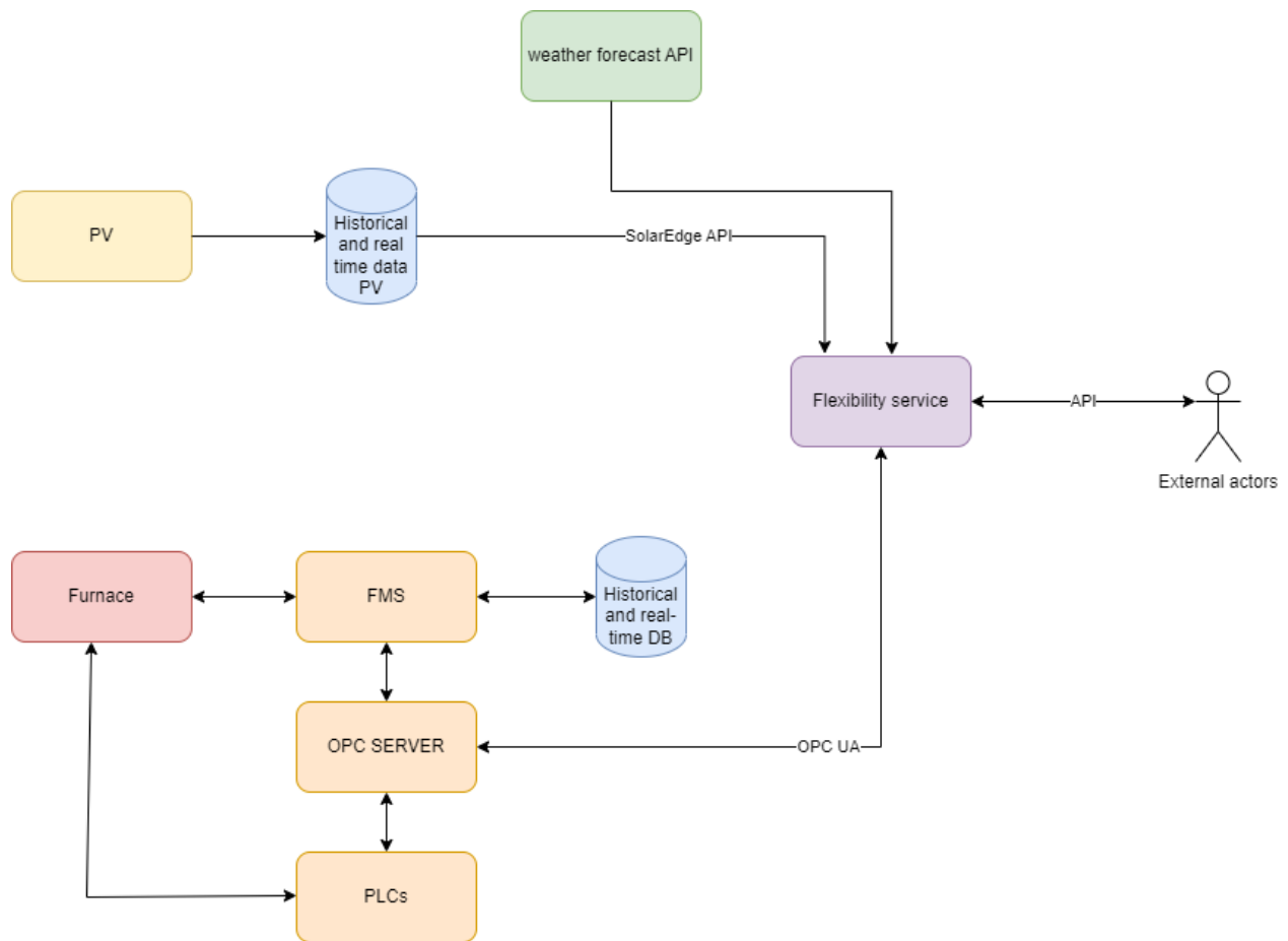
FIGURE 30: PILOT 1 ARCHITECTURE.
