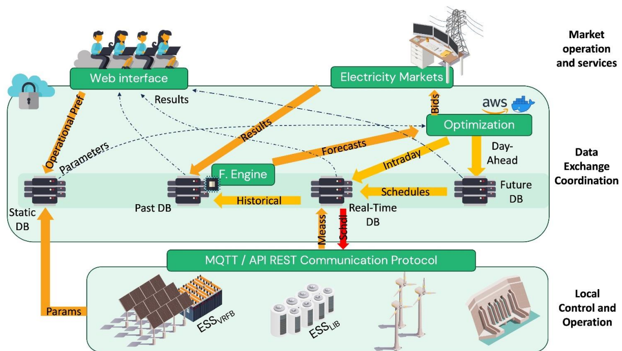
FIGURE 33: HOCS CONTROL LAYERS AND INTERACTIONS WITHIN THE CONTROL SYSTEM.
