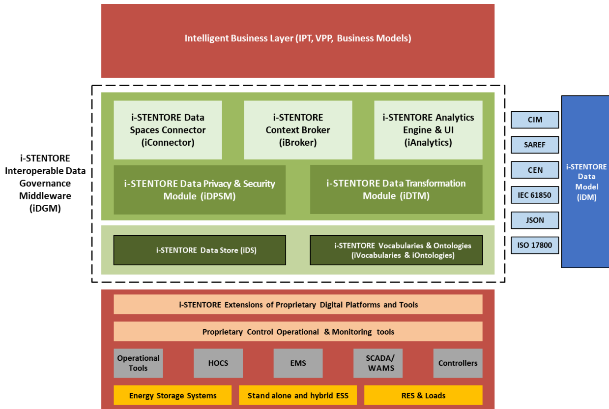
FIGURE 29: i-STENTORE DATA GOVERNANCE MIDDLEWARE DECOMPOSITION DIAGRAM (V1)
