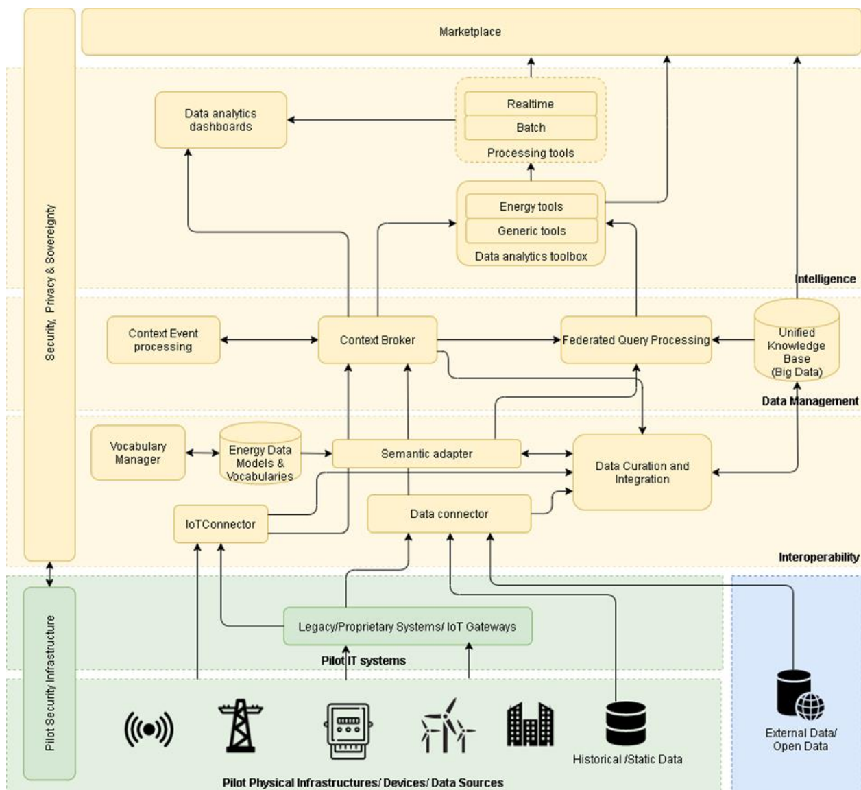
FIGURE 23: PLATOON REFERENCE ARCHITECTURE.
