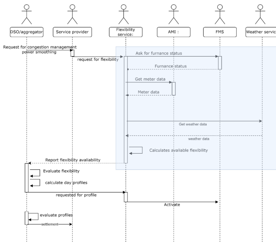
FIGURE 4: COMMUNICATIONS IN DEMO 1.
