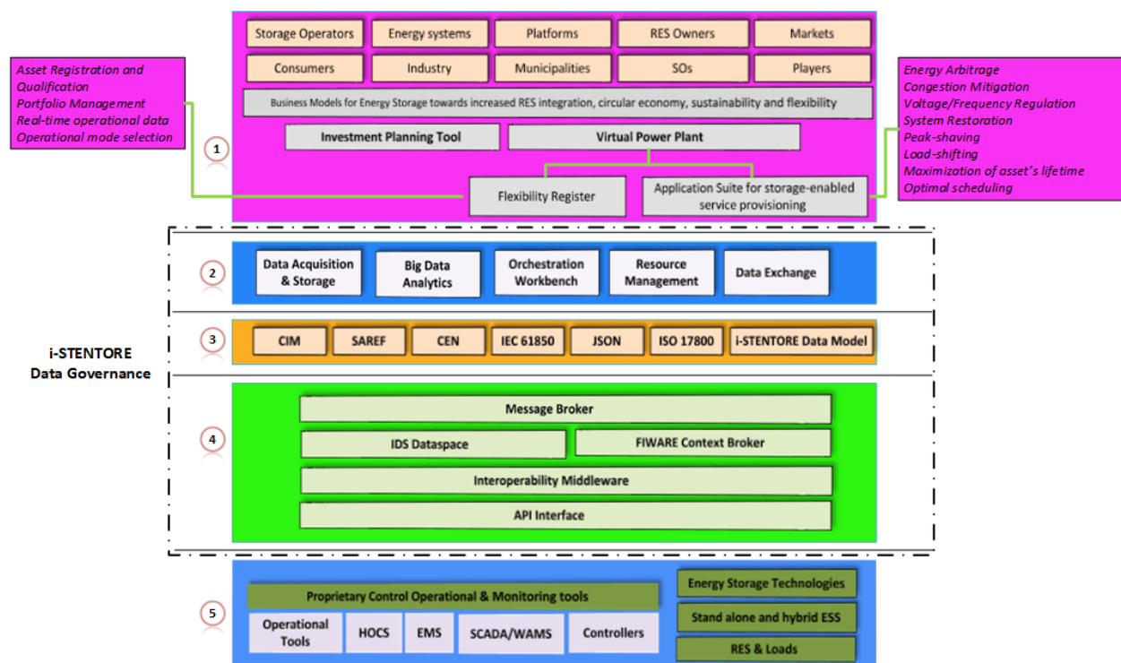
FIGURE 13: I-STENTORE SGAM REFERENCE ARCHITECTURE
