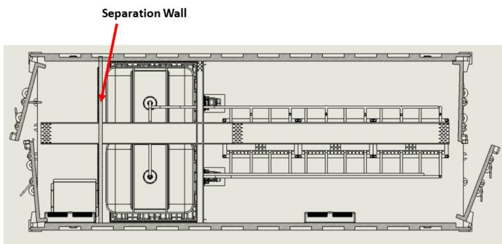
FIGURE 31: VRFB INSTALLATION LAYOUT.
