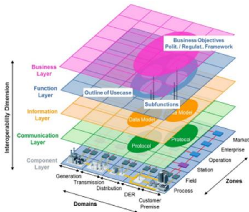
FIGURE 11: THE ORIGINAL SMART GRID ARCHITECTURE MODEL (SGAM). 5
