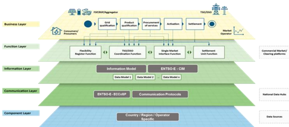
FIGURE 20: SGAM-BASED IEGSA ARCHITECTURAL REPRESENTATION.
