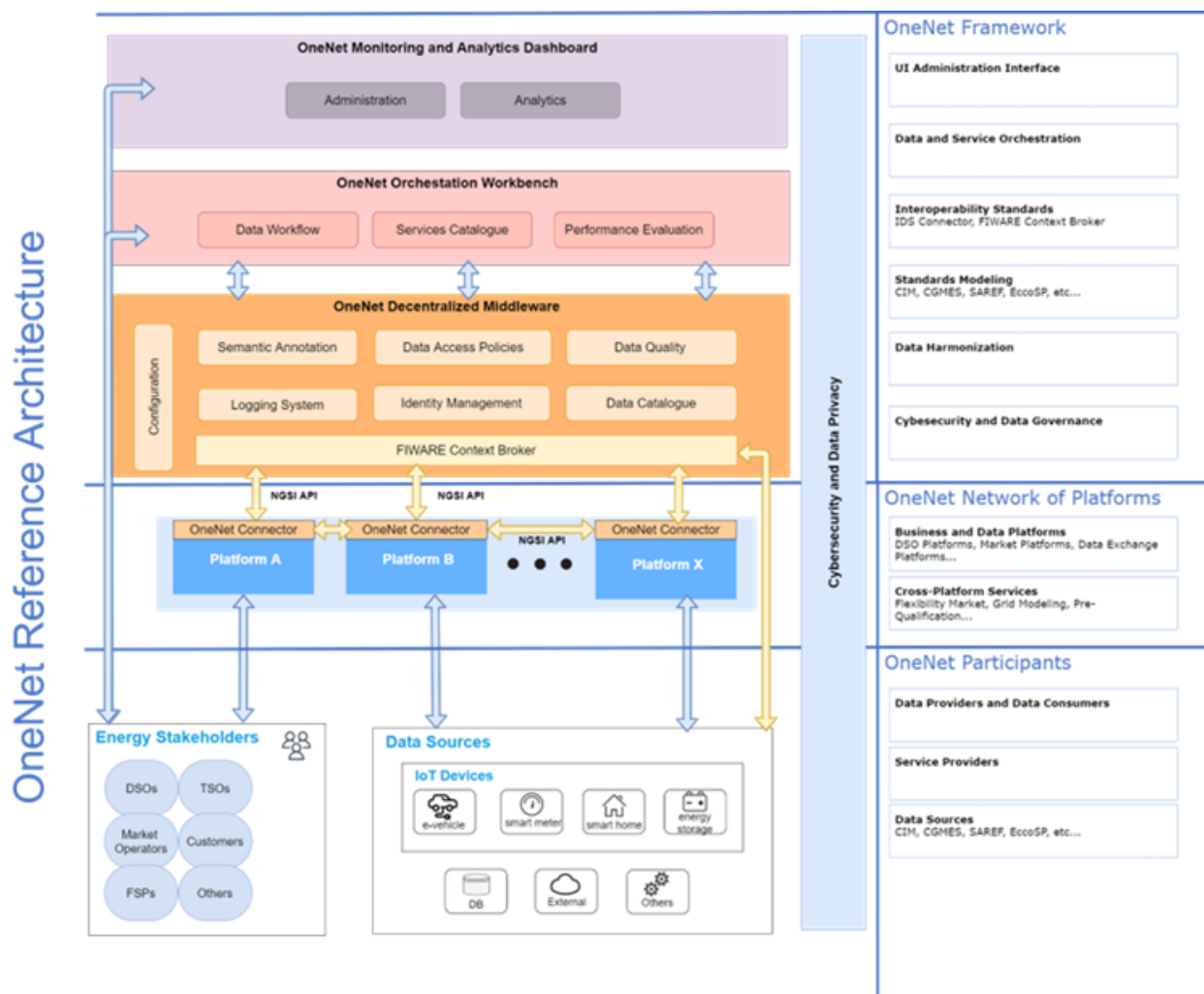
FIGURE 21: THE ONENET REFERENCE ARCHITECTURE.
