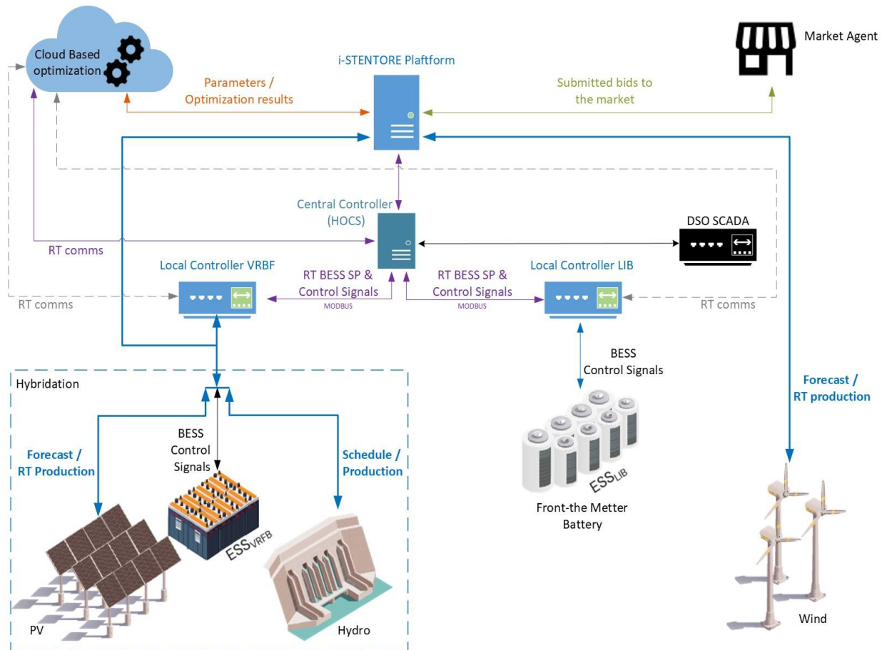
FIGURE 6: DATA SHARING IN DEMO 3.
