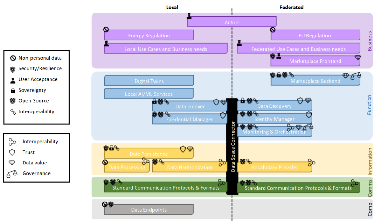
FIGURE 12: DERA 3.0 LAYERED ARCHITECTURE 7
