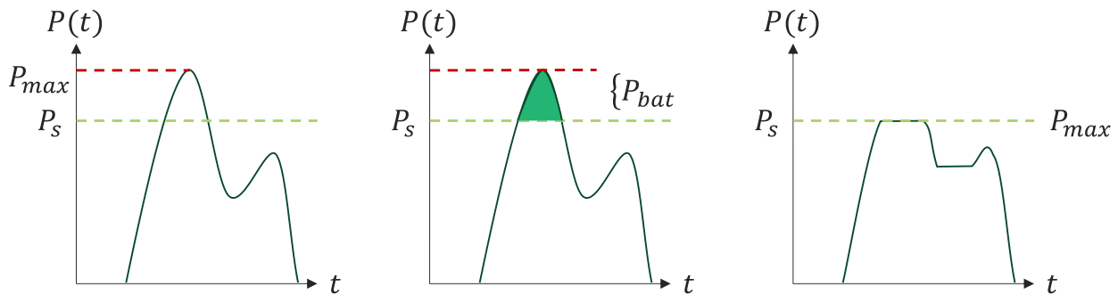
FIGURE 3: SCHEMATIC PEAK SHAVING OPERATION OF BATTERY STORAGE SYSTEM.
