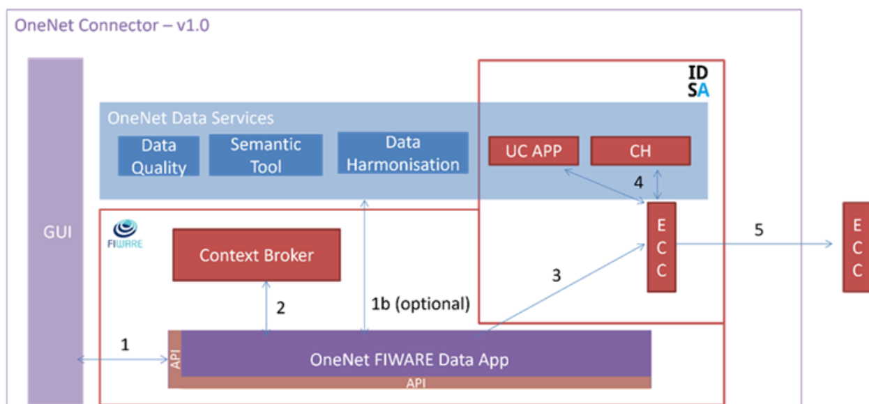
FIGURE 22: THE ONENET CONNECTOR ARCHITECTURE.
