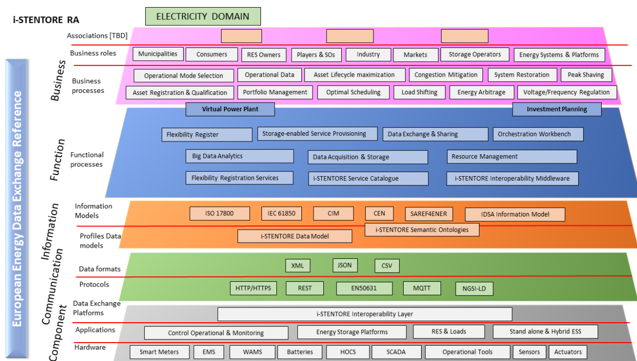
FIGURE 14: i-STENTORE BRIDGE REFERENCE ARCHITECTURE
