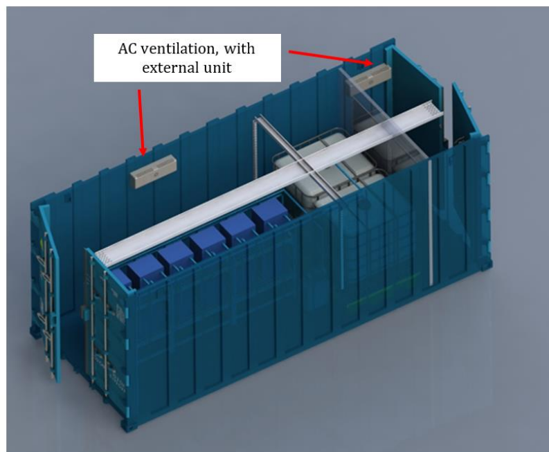
FIGURE 32: 3D VIEW OF THE VRFB CONTAINER LAYOUT.
