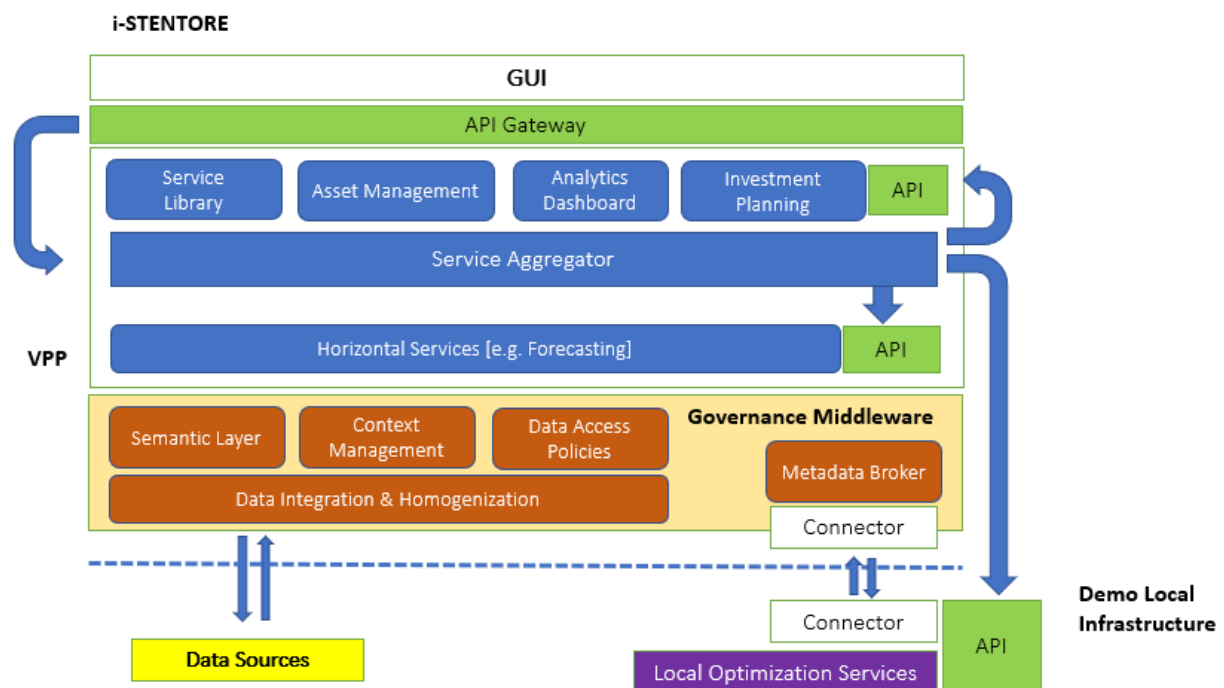
FIGURE 38: THE I-STENTORE HIGH-LEVEL S/W RA.
