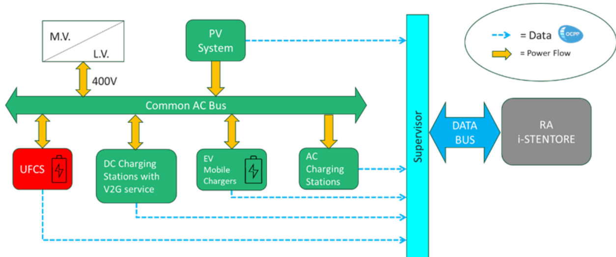
FIGURE 34: GLOBAL DEMO 4 PLANT SCHEME.
