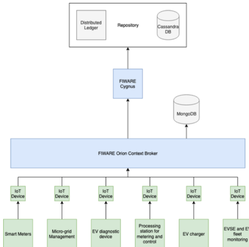
FIGURE 16: FIWARE'S ARCHITECTURE AND THE ROLE OF SMART-METER AGGREGATOR. 10
