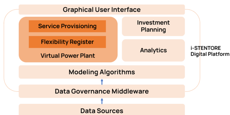
FIGURE 26: ESS-VPP COMPONENT STATIC VIEW.
