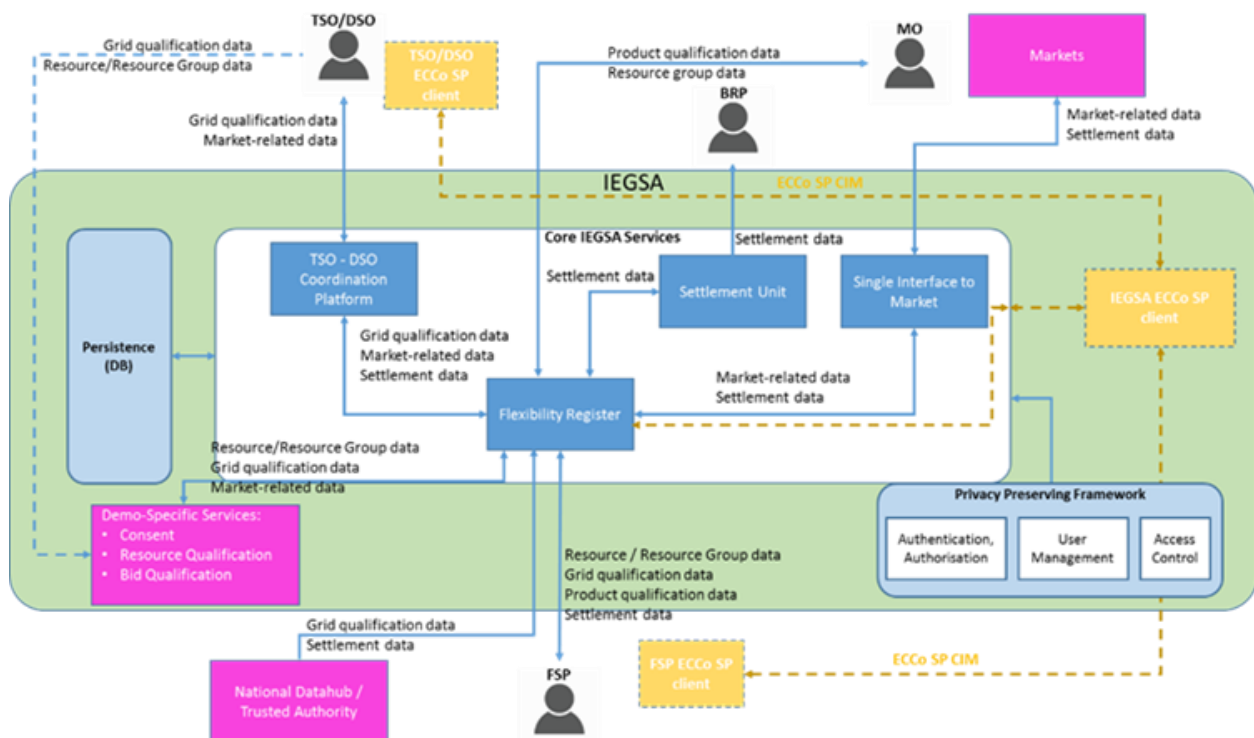
FIGURE 19: IEGSA LOGICAL ARCHITECTURE.
