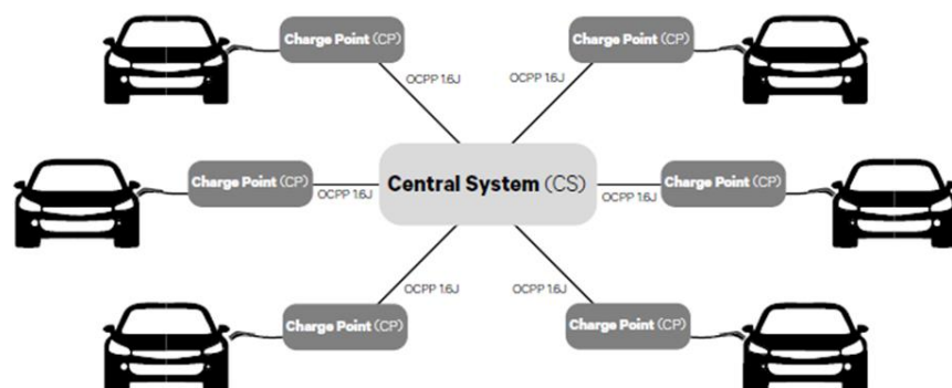
FIGURE 35: OCPP APPLICATION IN A GENERIC CHARGE INFRASTRUCTURE.
