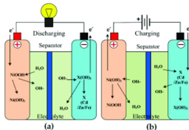
FIGURE 8: NICKEL BASED BATTERY SCHEME [23].
