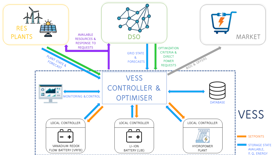
FIGURE 20: VESS ARCHITECTURE.
