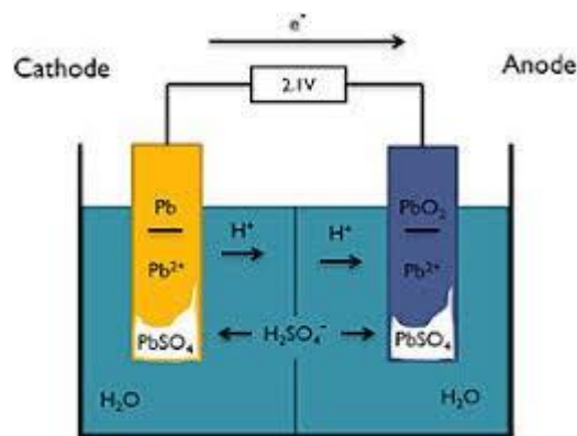
FIGURE 4: LEAD-ACID BATTERY SCHEME [12].
