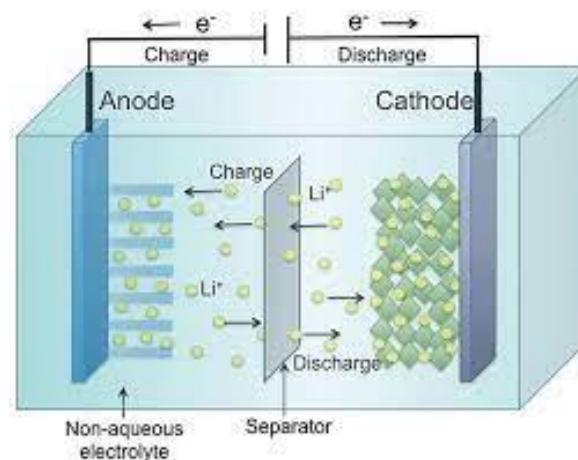
FIGURE 6: LITHIUM-ION BATTERY SCHEME [17].
