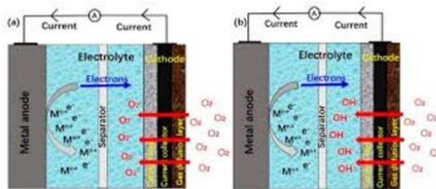
FIGURE 7: METAL-AIR BATTERY SCHEME [20].
