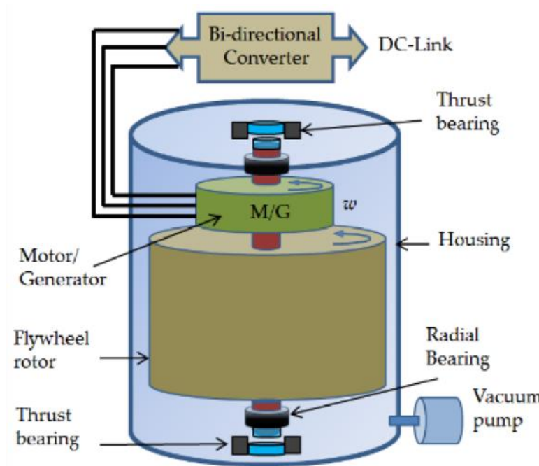
FIGURE 3: STRUCTURE AND COMPONENTS OF A FLYWHEEL. [7].
