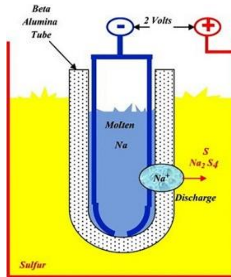
FIGURE 5: SODIUM-BETA BATTERY SCHEME [14].
