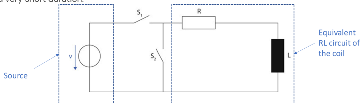
FIGURE 12: RL CIRCUIT REPRESENTED A SIMPLIFIED EQUIVALENT CIRCUIT FOR THE COIL WITH TWO SWITCHES [52].
