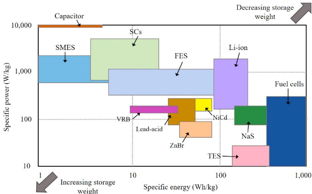
FIGURE 14 – RAGONE DIAGRAM SHOWING THE ENERGY DENSITY VERSUS POWER DENSITY OF DIFFERENT ESS TECHNOLOGIES [54].
