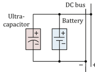
FIGURE 21: PASSIVE HYBRID ENERGY STORAGE SYSTEM [103].
