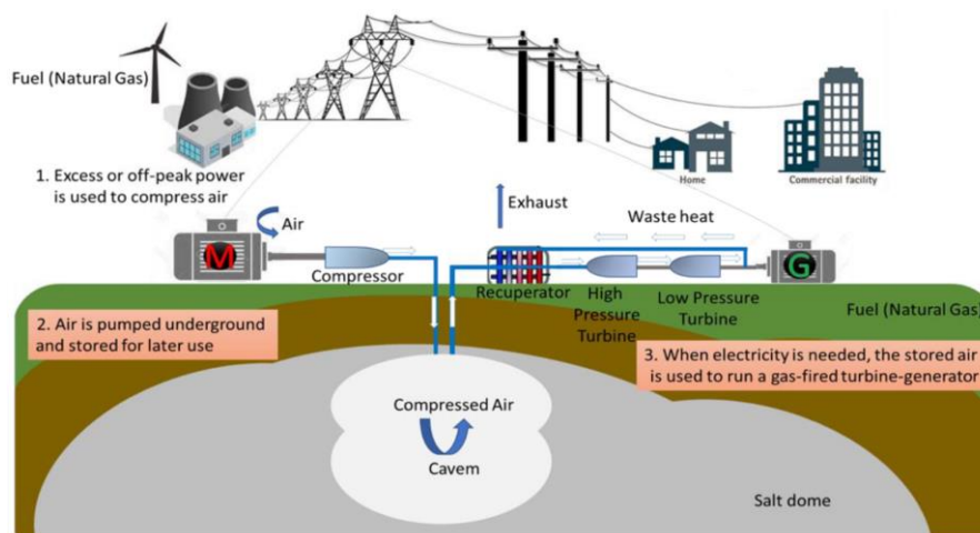
FIGURE 18: COMPONENTS OF THE CAES SYSTEM [66].
