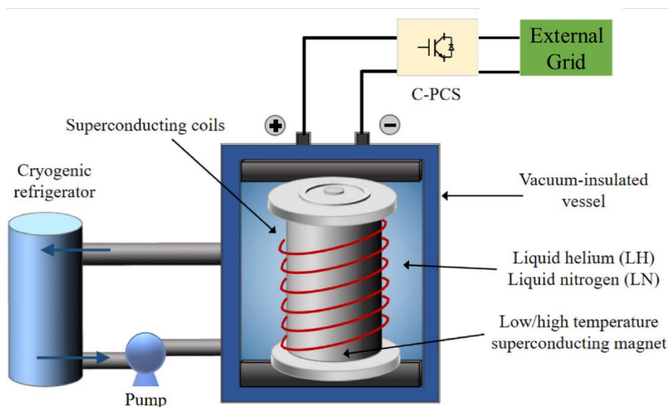
FIGURE 13: A SCHEMATIC DIAGRAM OF A SMES SYSTEM FOR GRID DISTRIBUTION [54].
