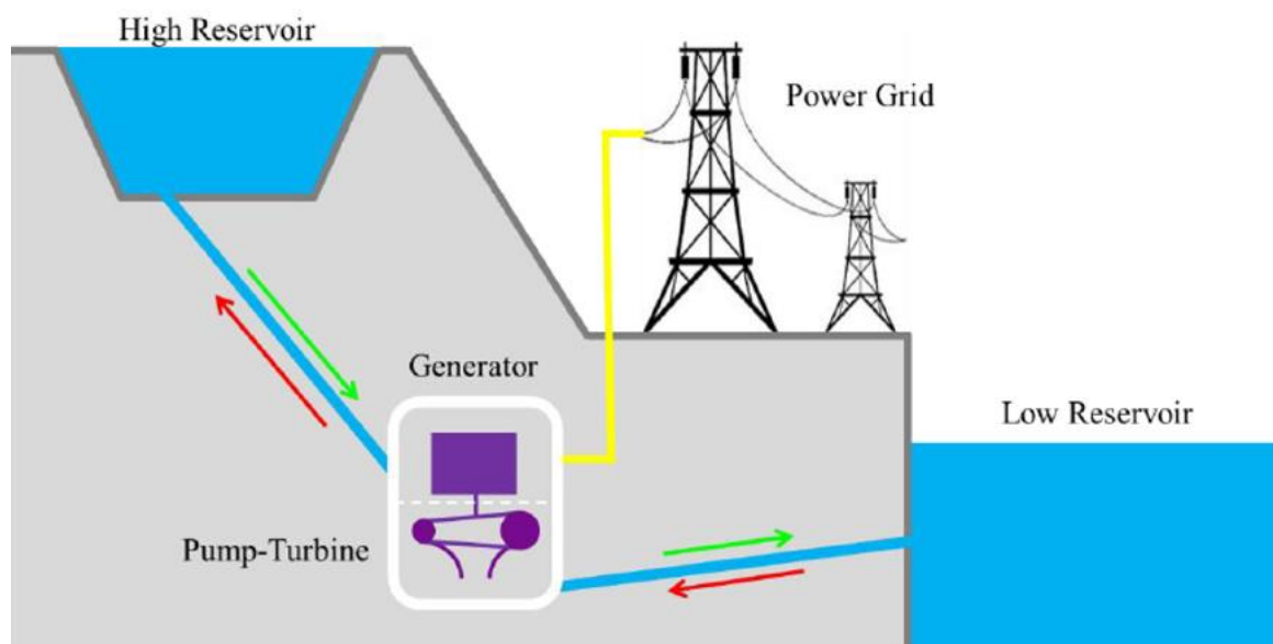
FIGURE 2: PUMPED HYDRO ENERGY PLANT, INCLUDING THE HYDRAULIC PUMP MODE AND TURBINE MODE [3].
