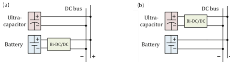
FIGURE 22: SEMI-ACTIVE HYBRID ENERGY STORAGE SYSTEM TOPOLOGY: (A) BATTERY SEMI-ACTIVE TOPOLOGY (B) ULTRA-CAPACITOR SEMI-ACTIVE TOPOLOGY [103].
