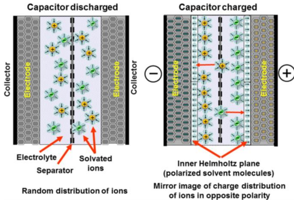
FIGURE 10: DIAGRAM OF A SYMMETRICAL ELECTROCHEMICAL CAPACITOR AT DISCHARGED AND CHARGED STATES [50].
