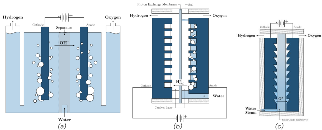
FIGURE 16: TYPES OF WATER ELECTROLYSIS. (A) AEL, (B) PEMEL, AND (C) SOEL [58].
