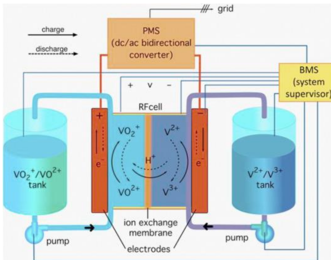
FIGURE 9: FLOW BATTERY SCHEME [26]
