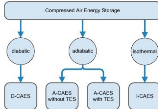
FIGURE 19: COMPRESSED AIR ENERGY STORAGE CONCEPTS CLASSIFIED BY THEIR IDEALIZED CHANGE OF STATE: (D(DIABATIC)-, A(ADIABATIC)-, I(ISOTHERMAL)-CAES) [68].
