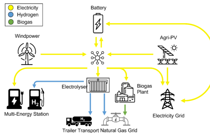
FIGURE 24: SCHEMATIC DIAGRAM OF THE HYBRID STORAGE SYSTEM COMBINING WINDPOWER, APV, A UTILITY-SCALE LI-ION BATTERY AND GREEN H 2 PRODUCTION AND STORAGE
