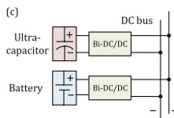
FIGURE 23: FULL-ACTIVE HYBRID ENERGY STORAGE SYSTEM TOPOLOGY [103].
