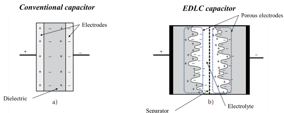
FIGURE 11: PRINCIPLE AND STRUCTURE OF CONVENTIONAL AND EDLC CAPACITORS [51].
